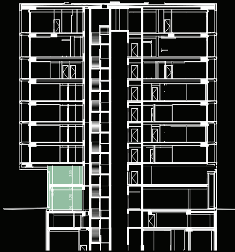
TRANSVERSAL SECTION
