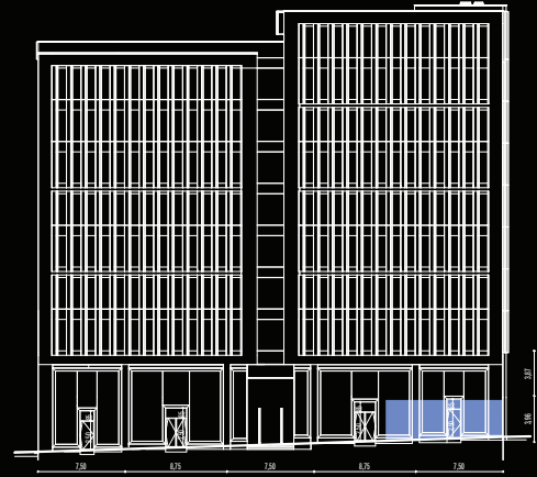
ELEVATION OF THE EAST FAÇADE
