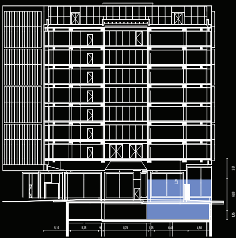
TRANSVERSAL SECTION
