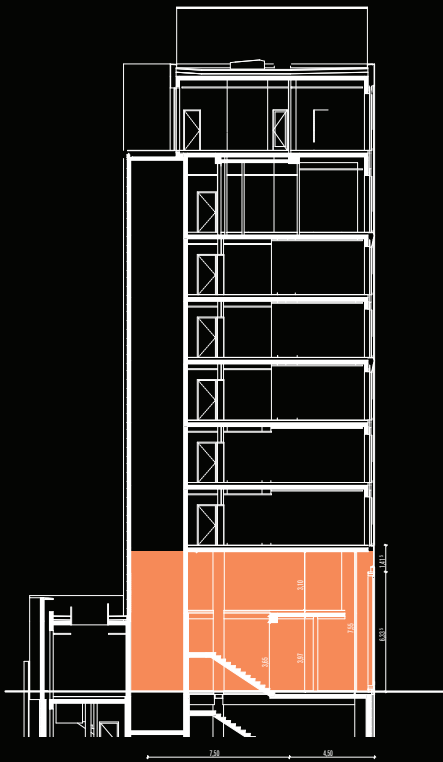
TRANSVERSAL SECTION
