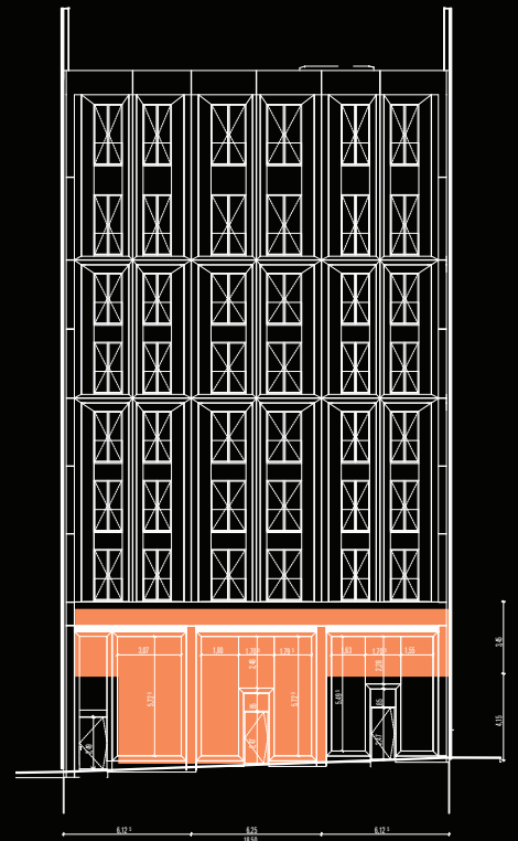
ELEVATION OF THE EAST FAÇADE
