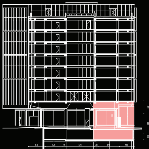
TRANSVERSAL SECTION
