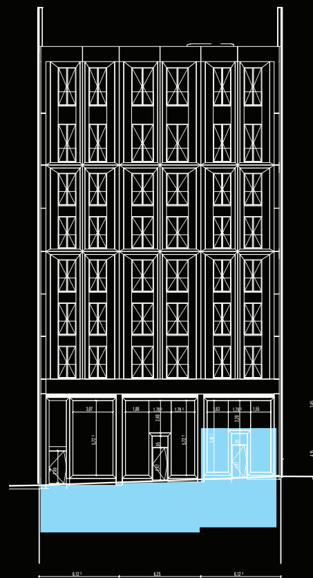
ELEVATION OF THE EAST FAÇADE
