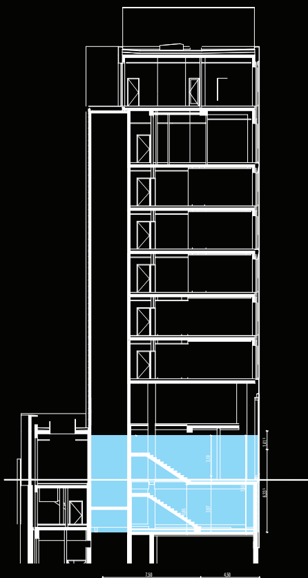
TRANSVERSAL SECTION
